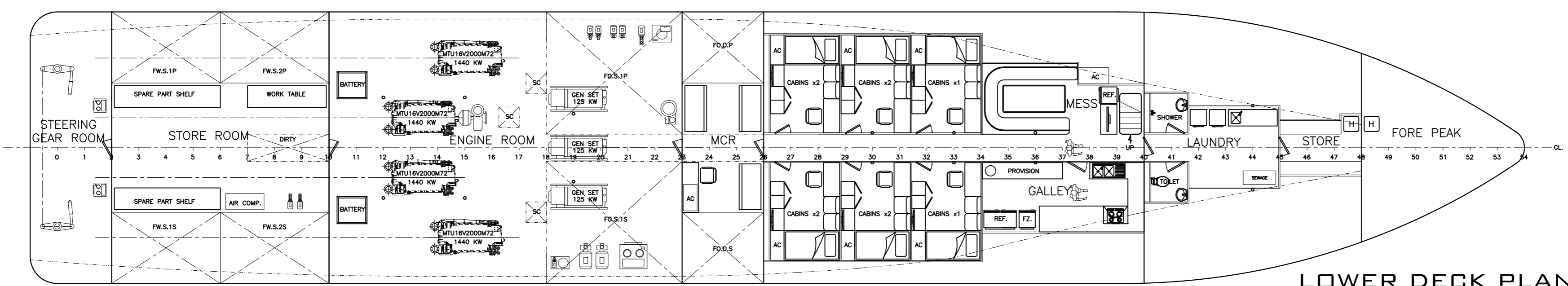
LOWER DECK PLAN
