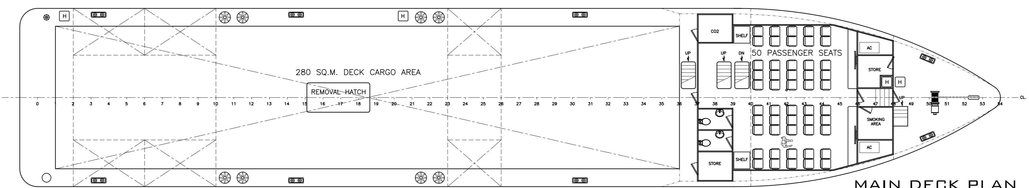
MAIN DECK PLAN
